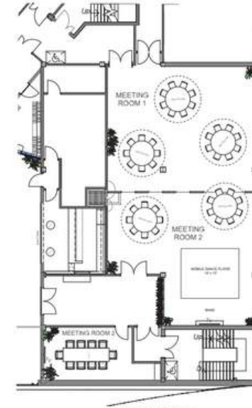
LAYOUT OPTION 03 - BANQUET STYLE WITH DANCE FLOOR Tables 1830 mm, 8 covers each COVERS - 40
